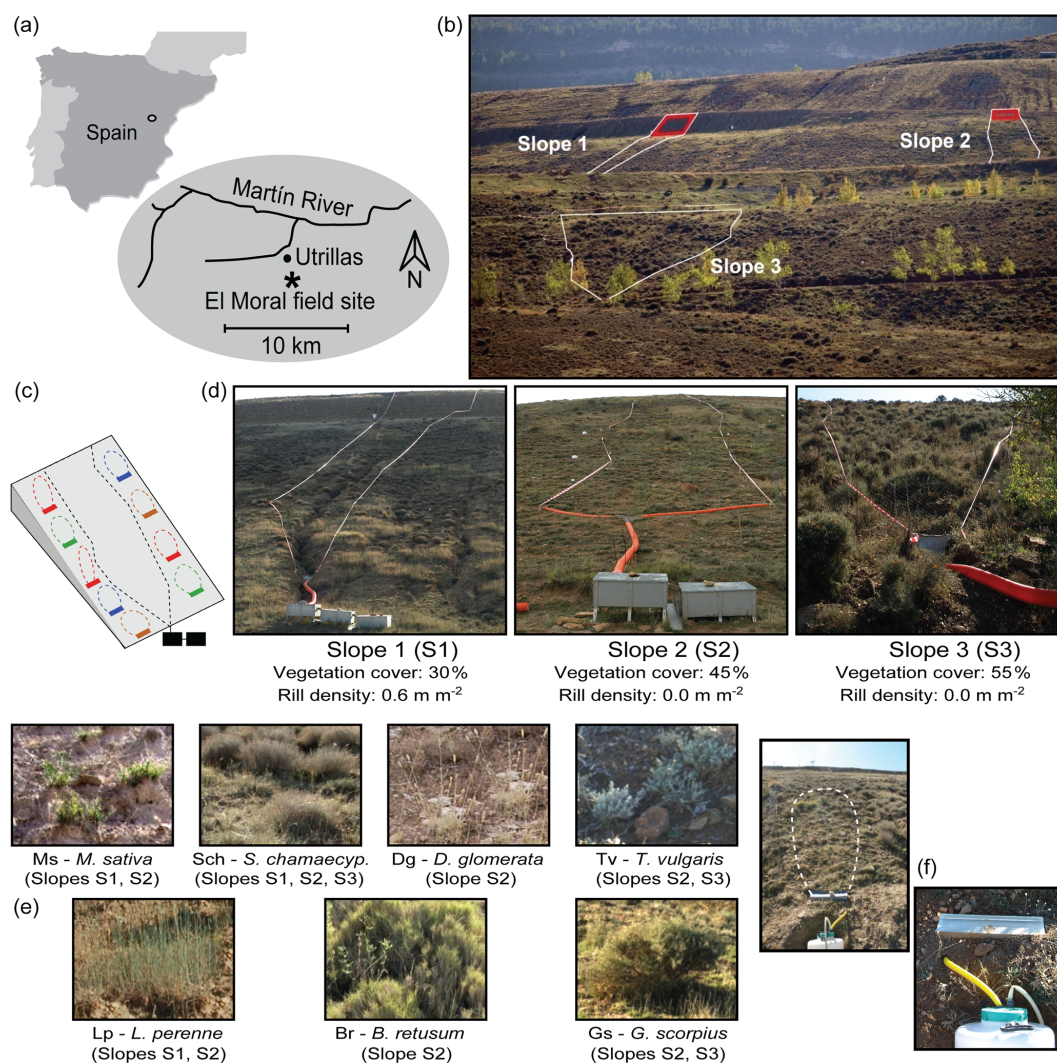
Figure 1. The Utrillas field site: (a) location map; (b) frontal view of the three experimental slopes (40° steep, berm sections located at the top of Slope 1 and Slope 2 are highlighted in red); (c) schematic representation of the experimental layout in the slopes (a hierarchical, scaled approach with patch-scale and hillslope-scale runoff and erosion plots); (d) frontal view of the hillslope-scale plots (catchment plots) and their general characteristics (vegetation cover and rill density); (e) detailed view of the seven surface types (vegetation communities) identified in the experimental slopes by Merino-Martín et al. (2012a); (f) an example of patch-size plot showing a small detail (right picture) of the Gerlach trough runoff and sediment collection systems. Names of the dominant plant species for the surface types: Ms, Medicago sativa ; Sch, Santolina chamaecyparissus ; Dg, Dactylis glomerata ; Tv, Thymus vulgaris ; Lp, Lolium perenne ; Br, Brachypodium retusum ; and Gs, Genista scorpius .
